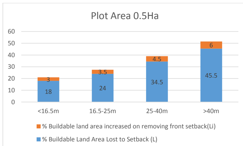
Figure 48 Buildable Area to Plot Size Comparison, Area 0.5Ha
