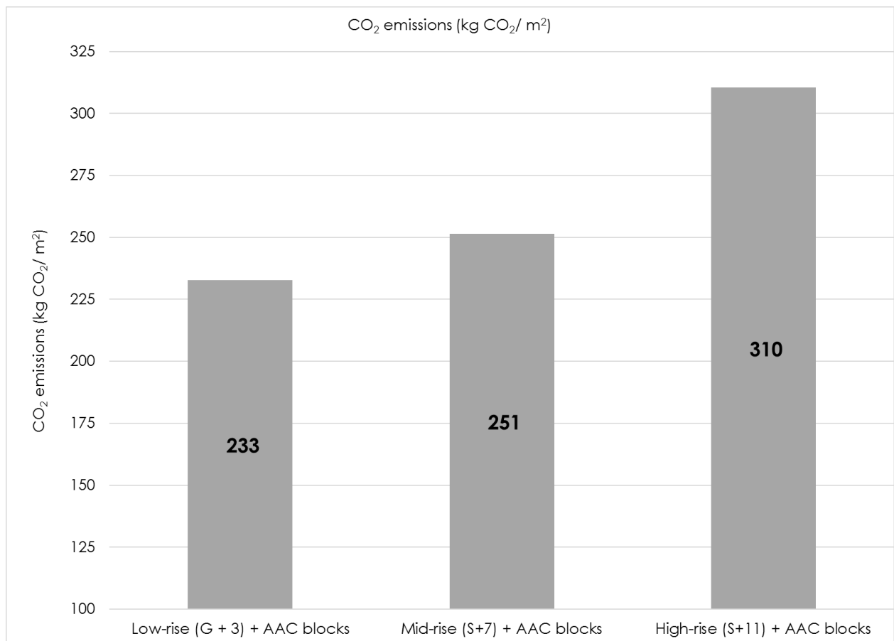
Figure 7 CO 2 emissions per m 2 built-up area from low-rise, mid-rise and high rise buildings
