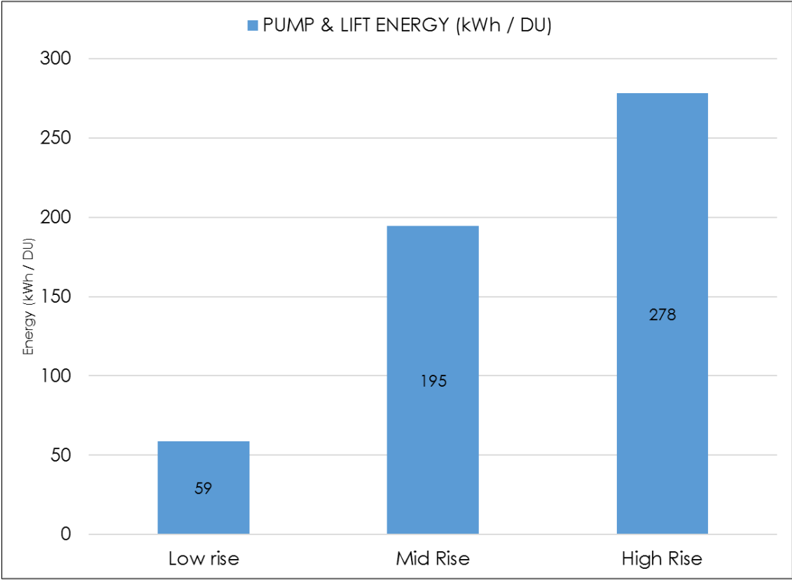
Figure 10: Comparison of pump and lift energy as per building height
