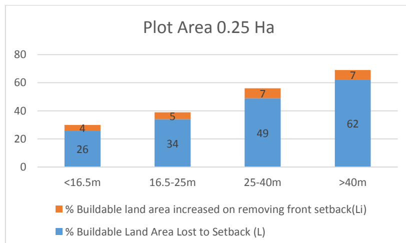
Figure 49 Buildable Area to Plot Size Comparison, Area 0.25 Ha
