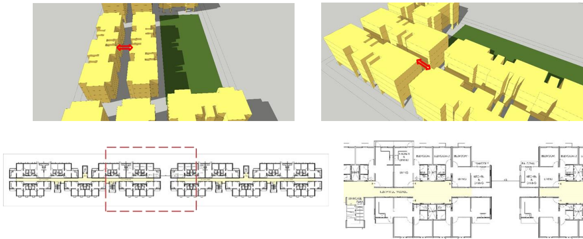
Figure 27 Building to building Margin and various configurations
