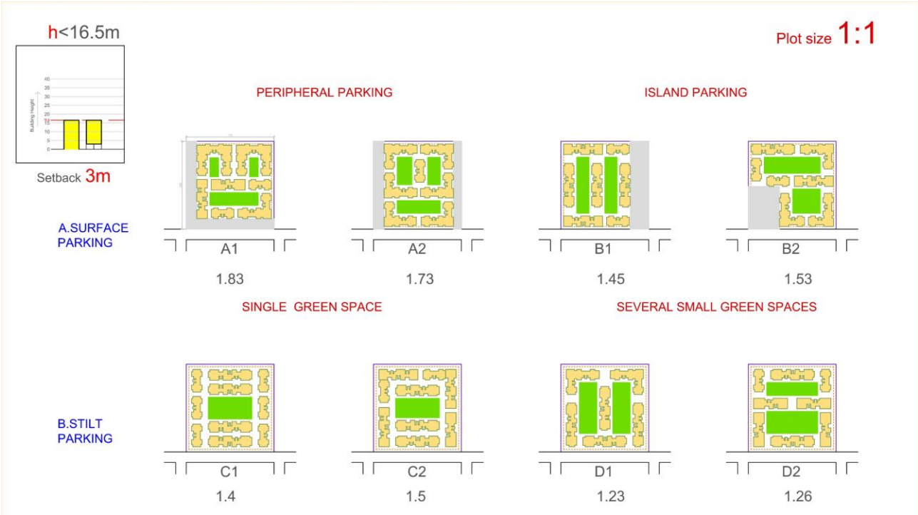
Figure 50 Spatial Configuration options for 1:1 type plot
