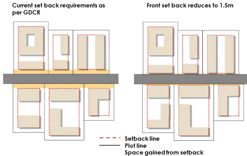
Figure 35 Reduction in Front Margin
