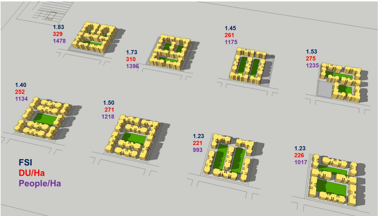
Figure 51 Comparison of various Spatial Configuration options for 1:1 type plot
