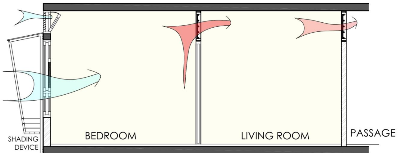
Figure 15 Cross Ventilation inside a House
