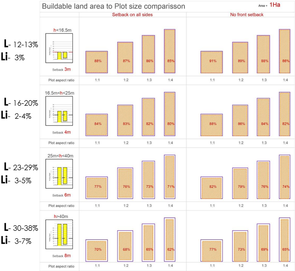
Figure 34 Buildable area to Plot size Comparison
