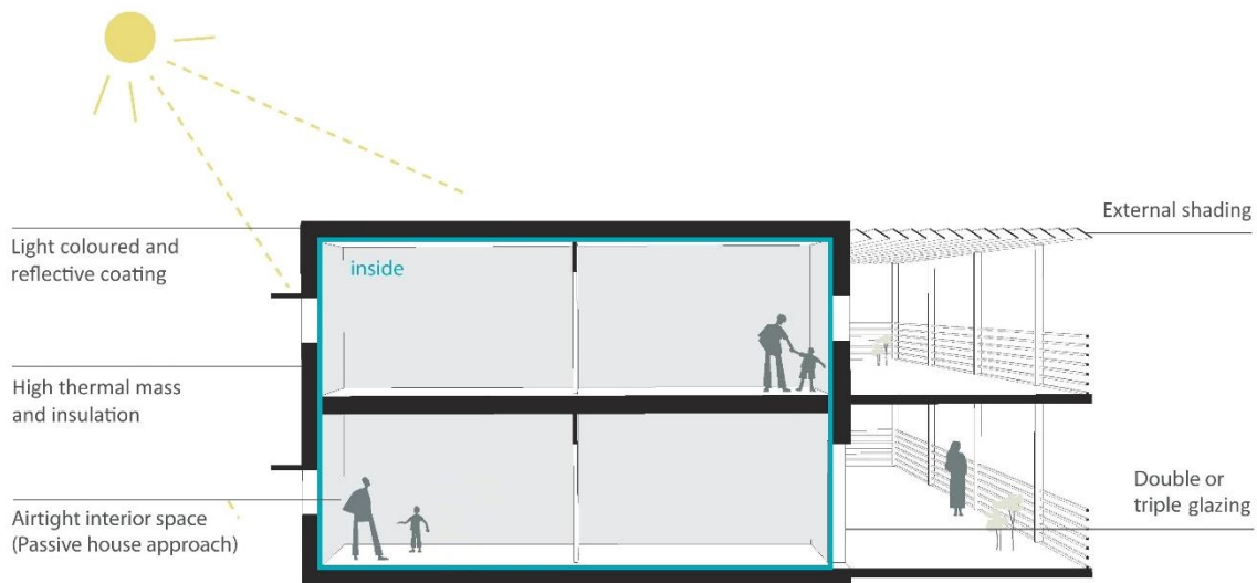
Figure 11: Closed building type in hot-dry climate (Source: PEEB, 2019)
