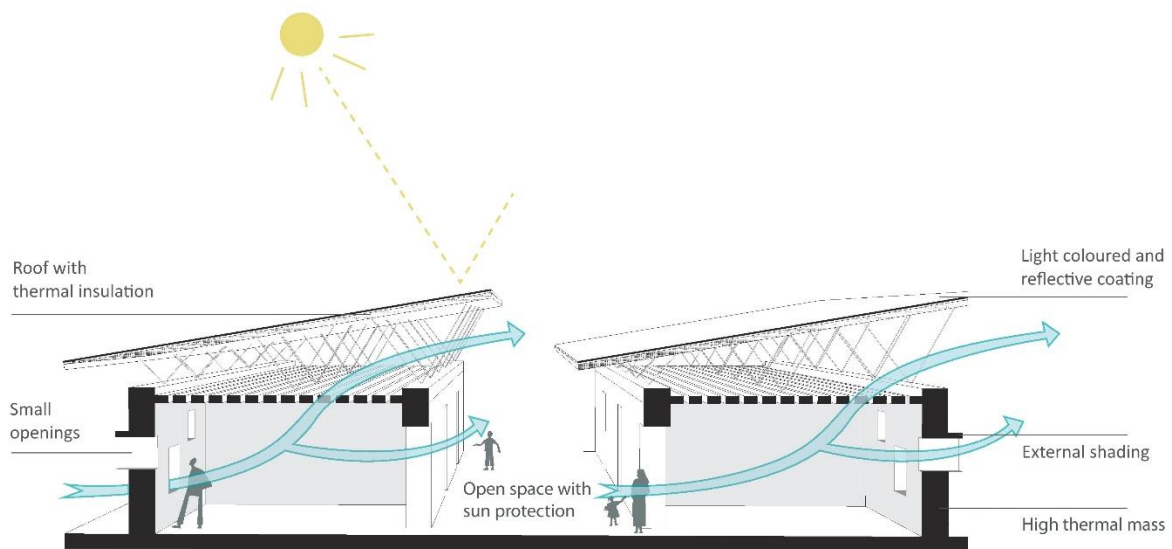
Figure 8: Open building type in hot-dry climates (Source: PEEB, 2019)
